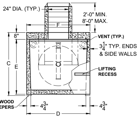
SECTION THRU "B-B"
